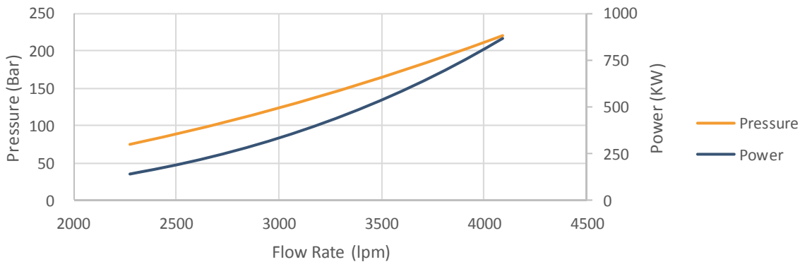
245-3D-97 Turbodrill Nominal Outputs with 1,2 SG WBM
