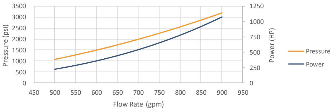
9-5/8"-3D-97 Turbodrill Nominal Outputs with 10ppg WBM
