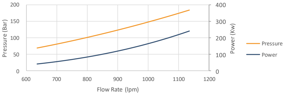
121-3D-120 Turbodrill Nominal Outputs with 1,2 SG WBM
