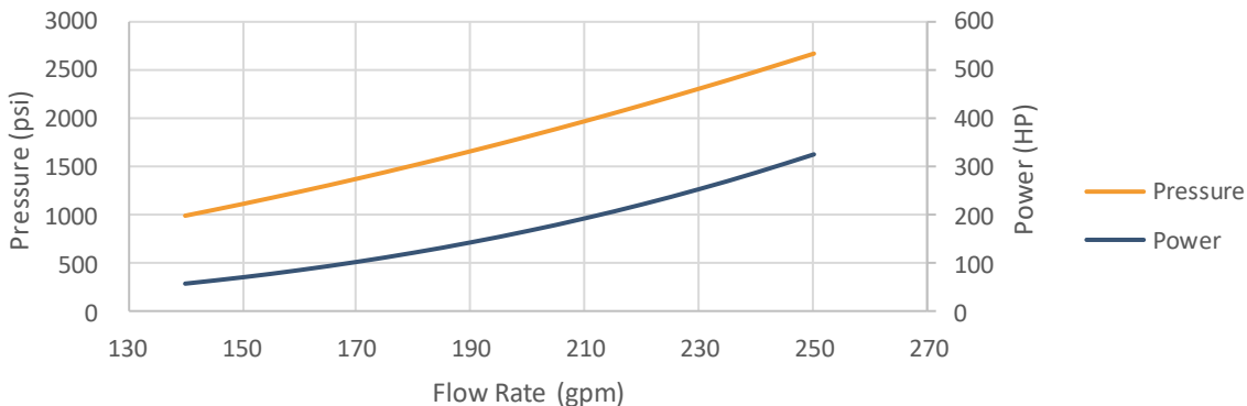
4-3/4"-3D-120 Turbodrill Nominal Outputs with 10ppg WBM
